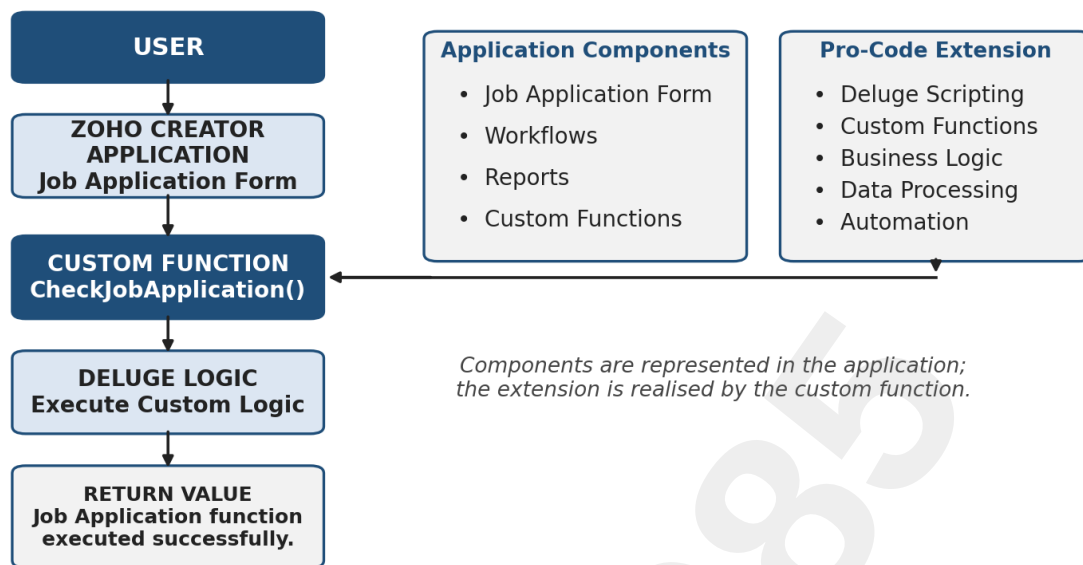
Figure 1: Pro-Code Extension of a Zoho Creator Application (Supporting Diagram)
